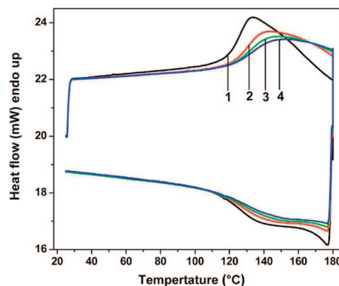
Figure 8. Thermal behavior of the cross-linked PK-furan (PK50f-1 at I_{\text{ma/fur}}/M_a = 1 ).
