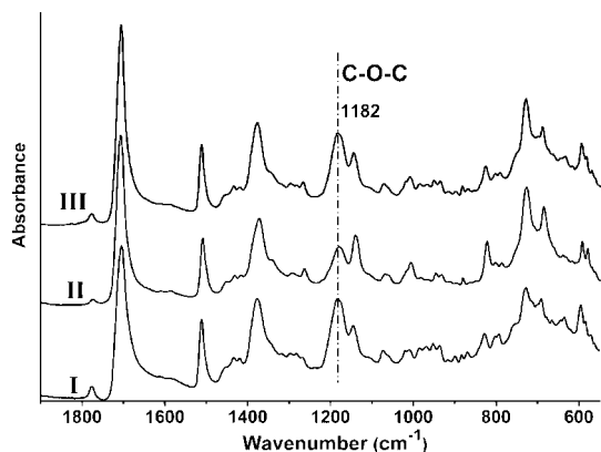
Figure 7. FTIR spectra of the cross-linked PK-furan (PK50f-1 at I_{\text{ma/fur}}/M_a = 1 ) before heat treatment at room temperature (I), upon heating to 150 °C for 5 min (II), and after cooling to room temperature in 20 min (III).
