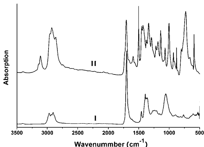
Figure 3. FTIR spectra of polyketones (PK50) (I) and furan-functionalized PK50 (II).
